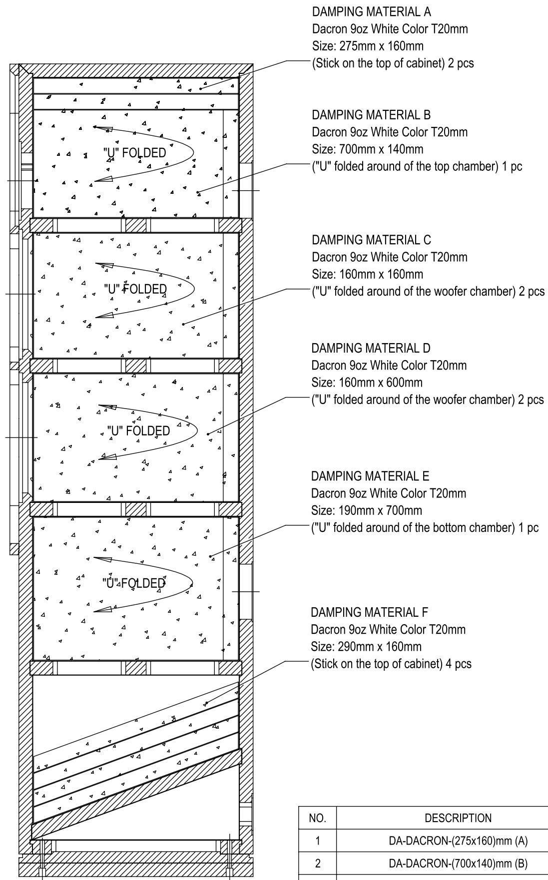
" SECTION VIEW "
