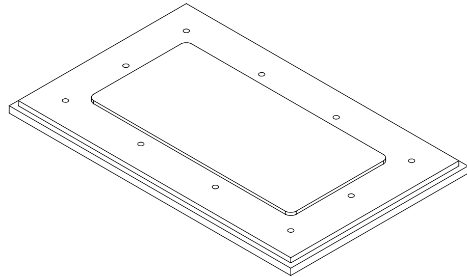
BOARD (G)
